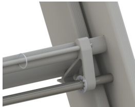
Block and tackle system with rope for easy & effective extension
