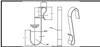
JUMBO Fall Protection Holder 100KS1102
